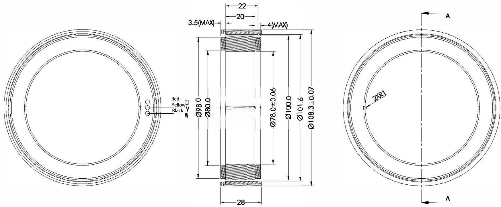
Cross-section A-A
