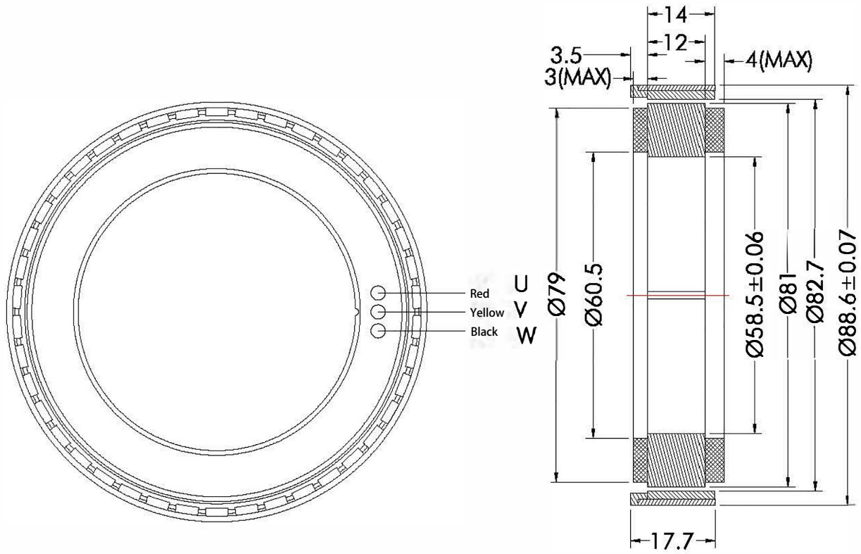
Cross-section A-A
